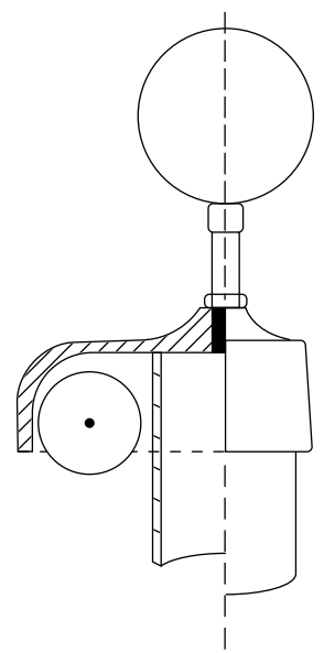
Stationary Truck Detail Cast Aluminum Body
